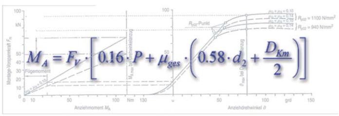
Kellermann-Klein formula by KAMAX The global standard for calculating bolted joints
